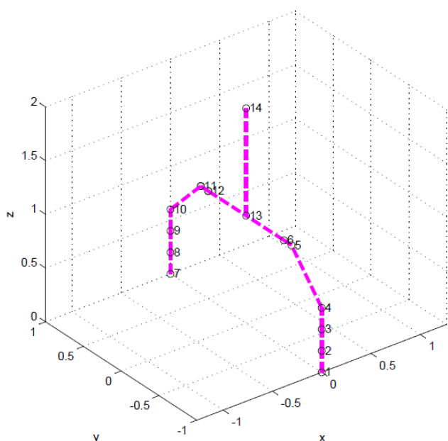
MECHDYN™ structural model: example of rigid fork
