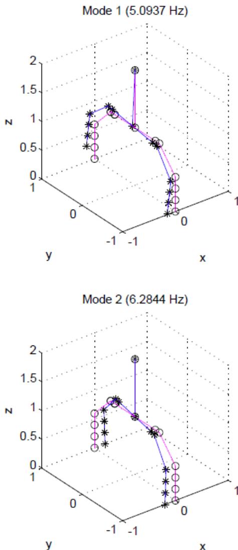
MECHDYN™ result plots: undeformed structure (magenta) and vibrating modes (blue)
